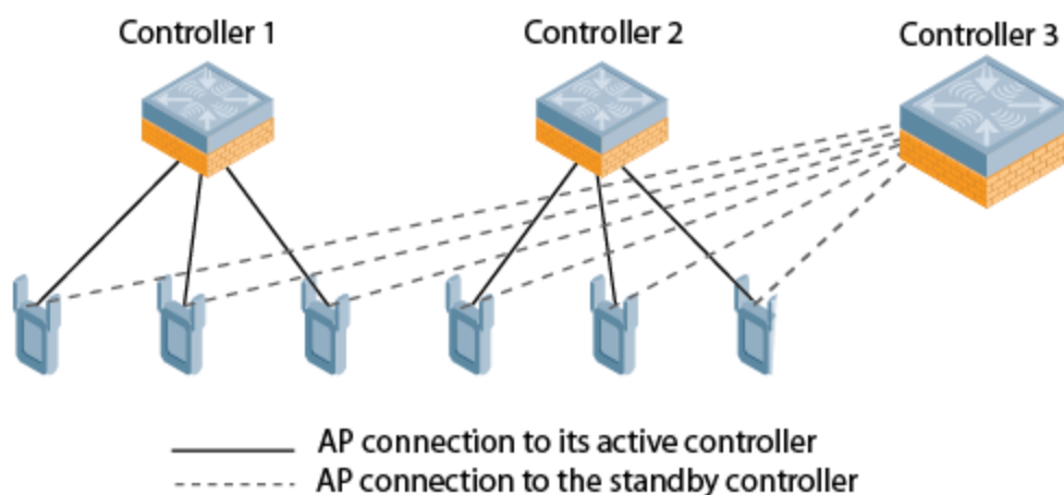
Figure 44 1:1 Active/Standby Deployment
