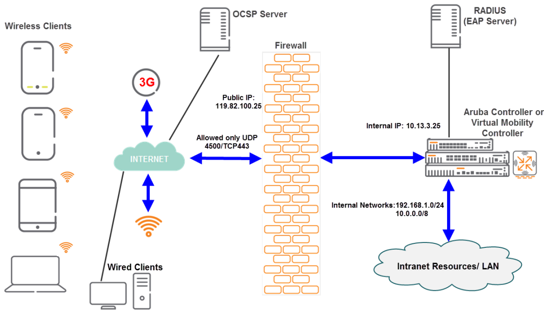
Figure 64 VIA Topology
