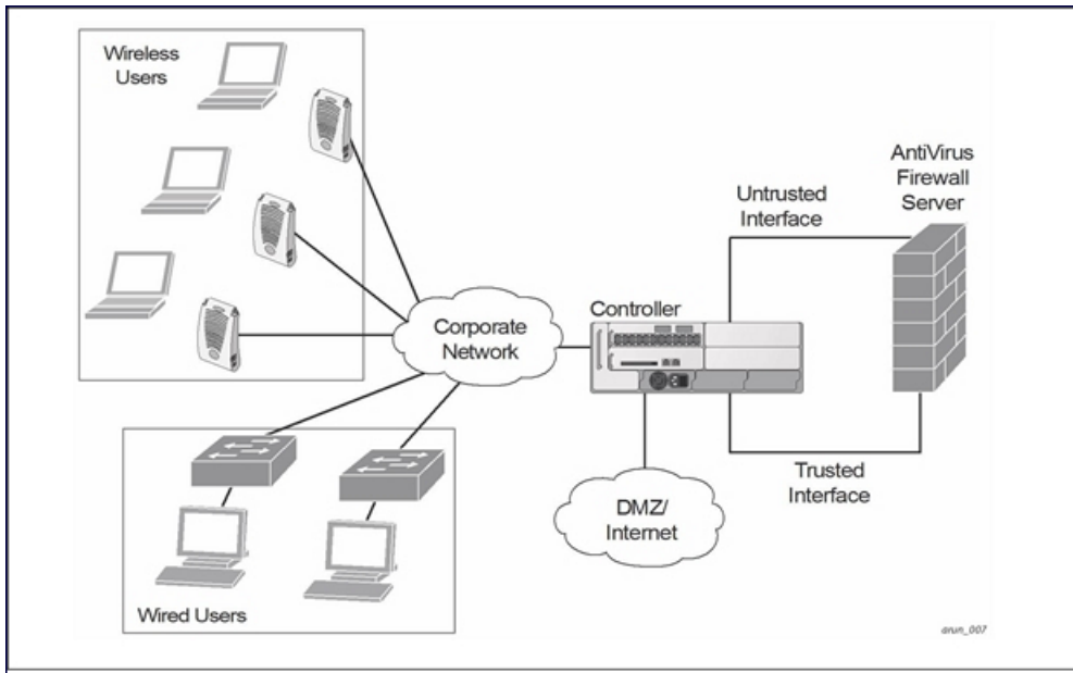
Figure 133 ESI-Fortinet Topology
