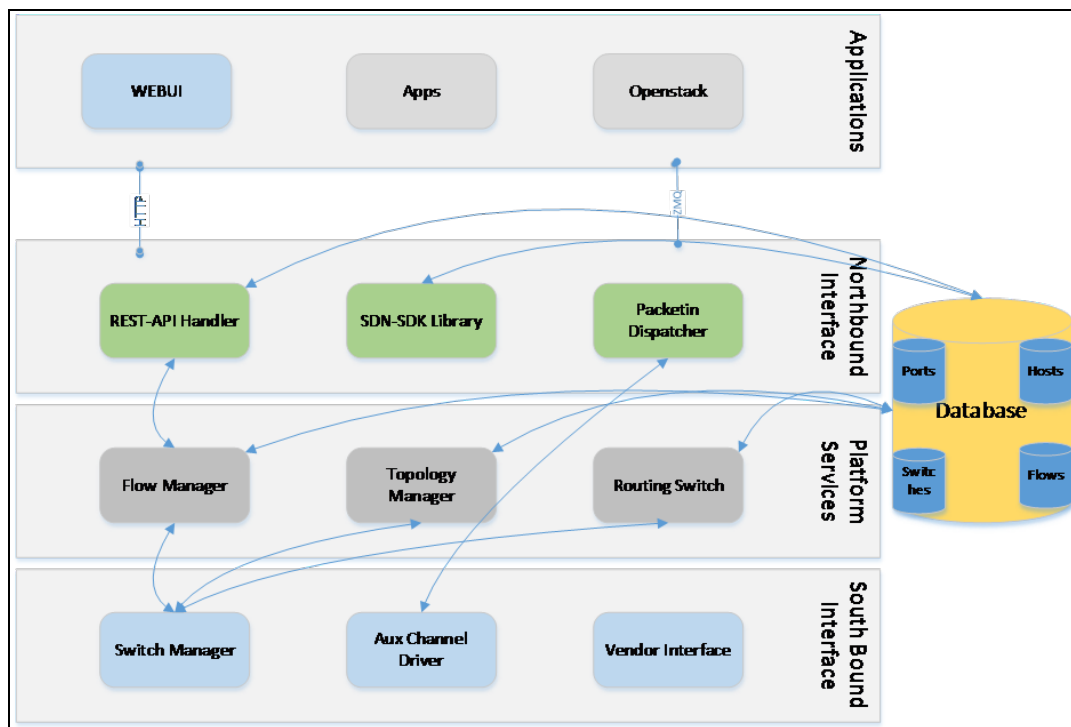
Figure 120 SDN Controller Architecture
