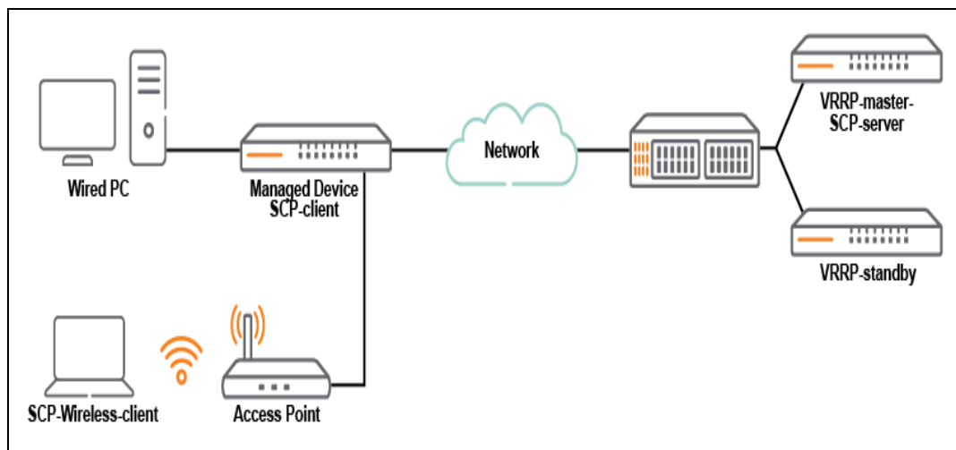
Figure 119 Sample Topology - VRRP Master as SCP Server
