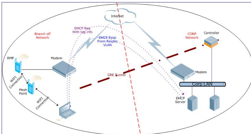
Figure 37 Working of Remote Mesh Portal
