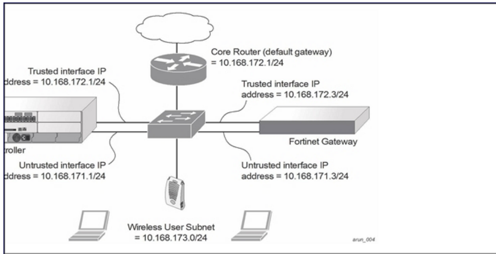
Figure 137 Example Route-Mode Topology
