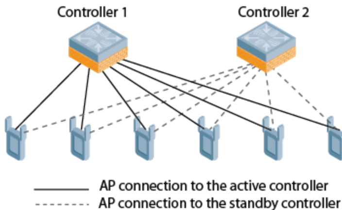
Figure 43 1:1 Active/Standby Deployment
