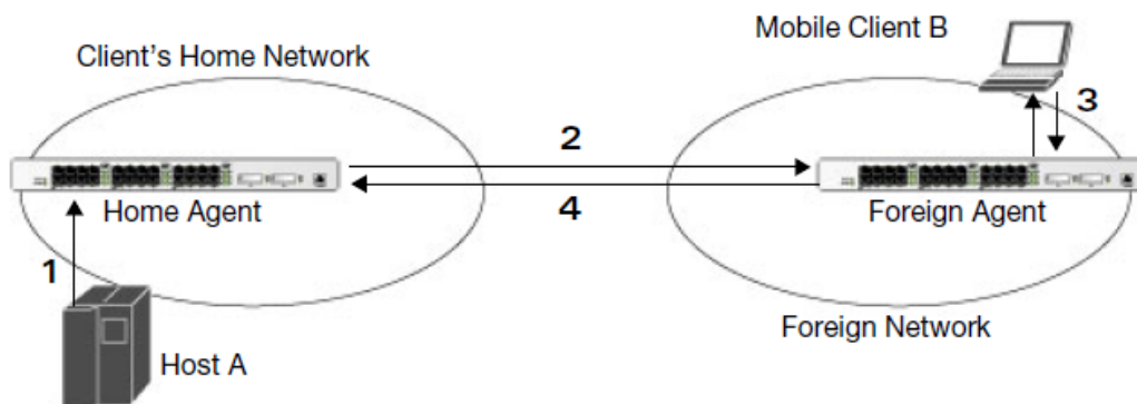
Figure 46 Routing of Traffic to Mobile Client within Mobility Domain
