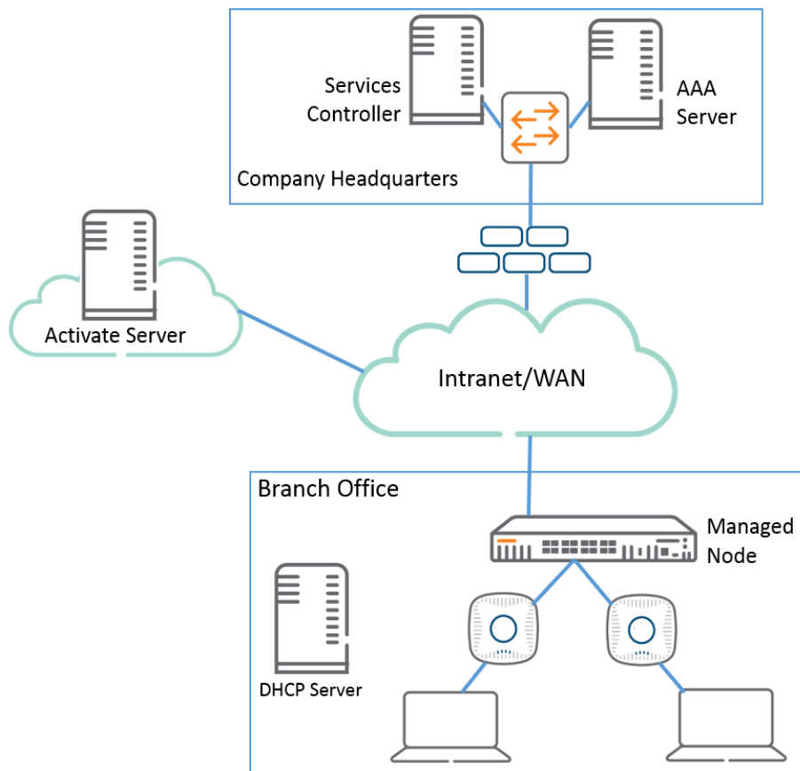
Figure 23 Managed Device Topology
