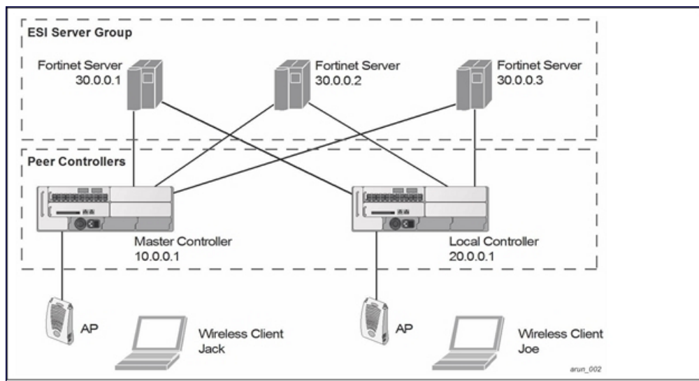
Figure 136 ESI Peer managed device
