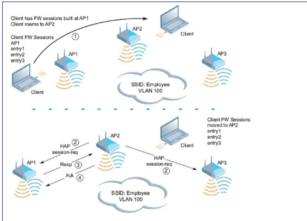
Figure 48 Bridge Mode Mobility
