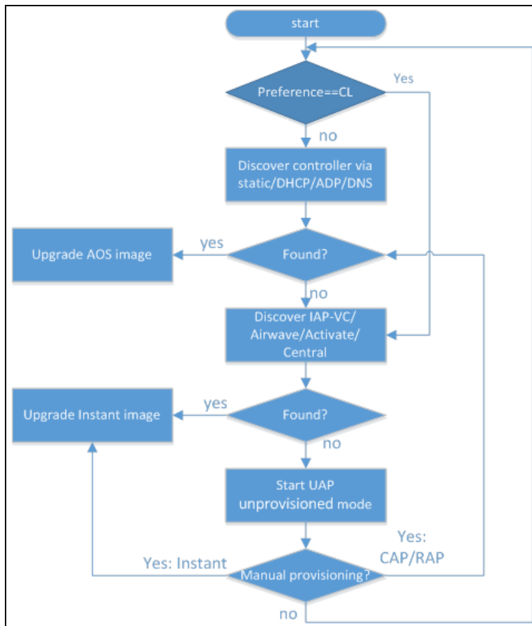
Figure 35 AP Discovery Logic
