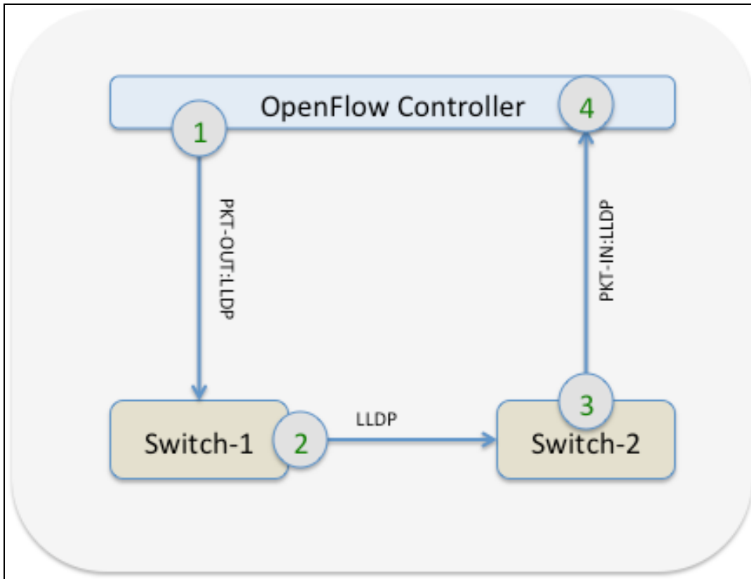
Figure 121 Topology Discovery
