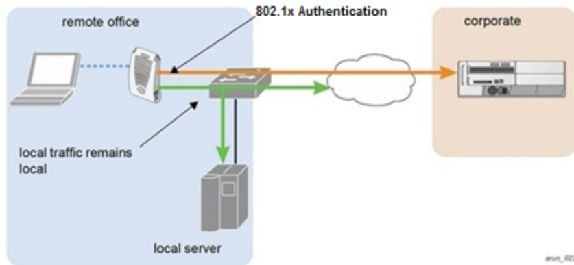
Figure 53 Sample Bridge Environment
