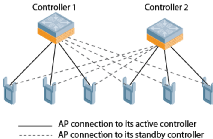
Figure 42 Active-Active HA Deployment
